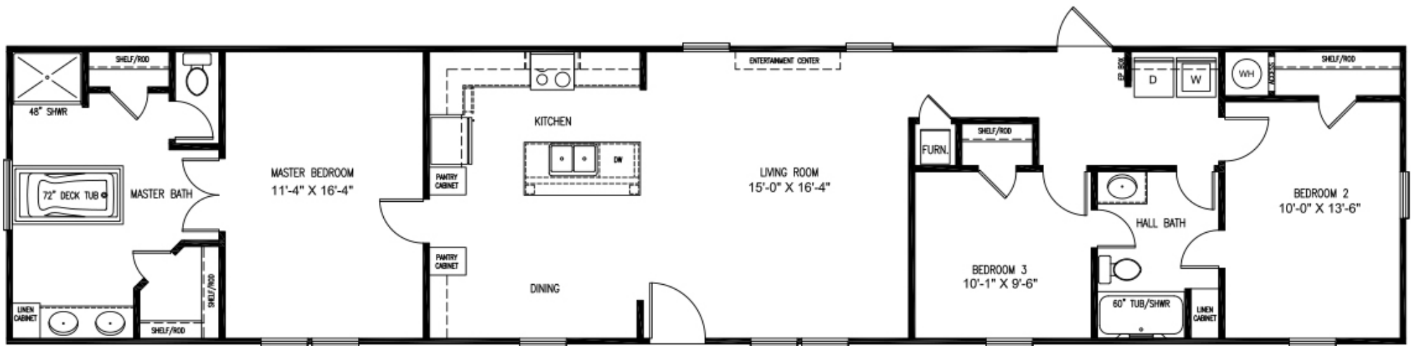
MODEL # NV-1802 18' X 80' DIMAS
