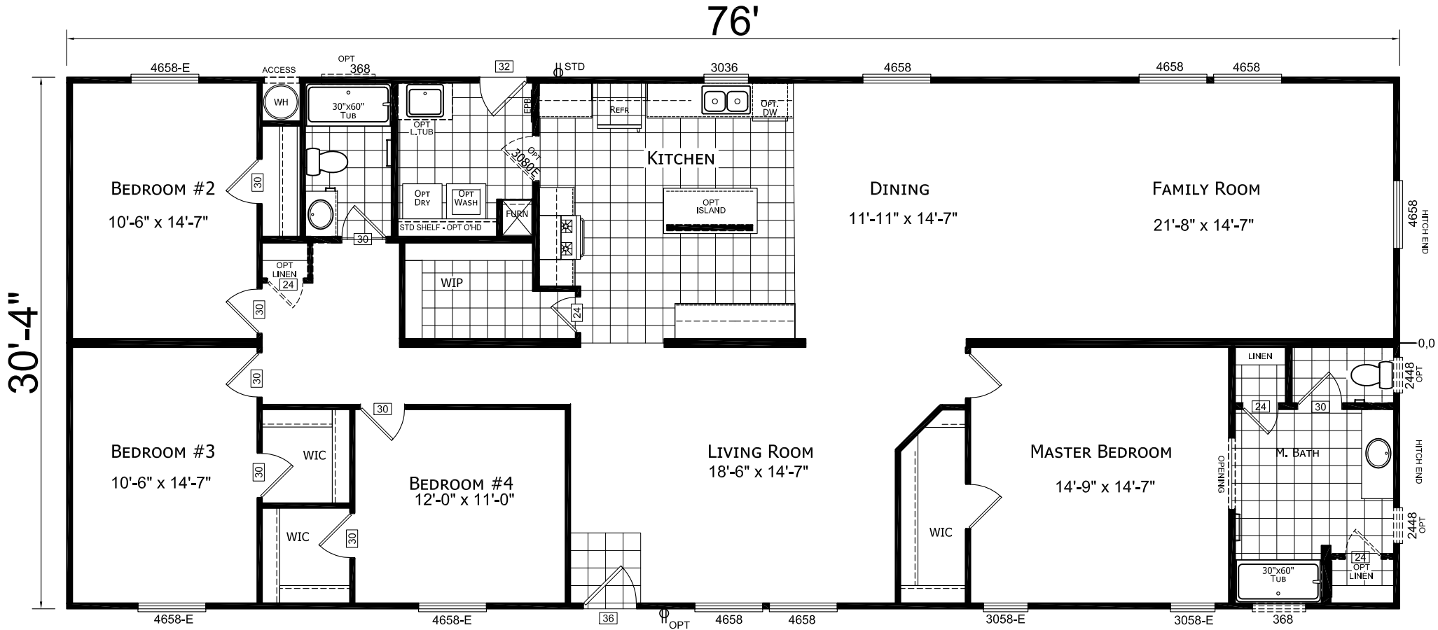
MODEL AF3276B TOTAL AREA: 2305 SQ. FT. 4 BEDROOM, 2 BATH REVISED 03/21/2020
